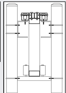
EasyGlide Dual Track Gate
